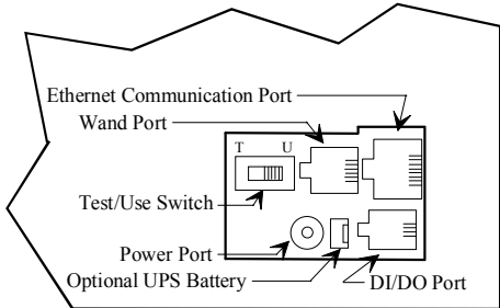
(Sectional Cut-out of the Terminal Chassis)
