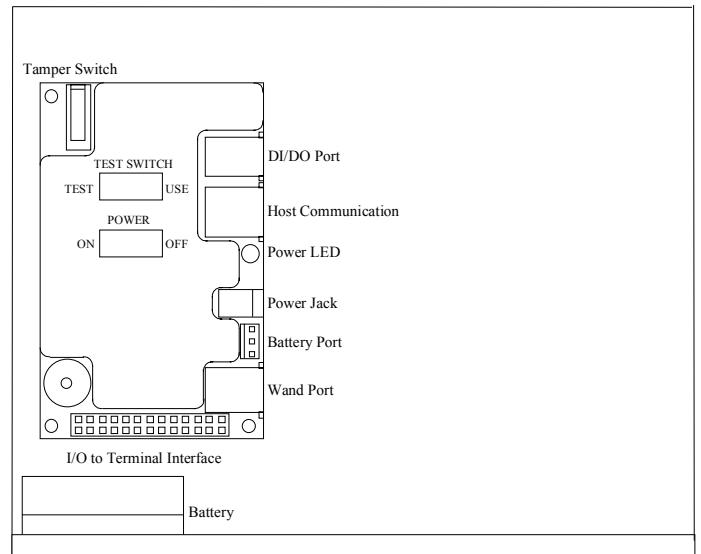
(Base Assembly)
